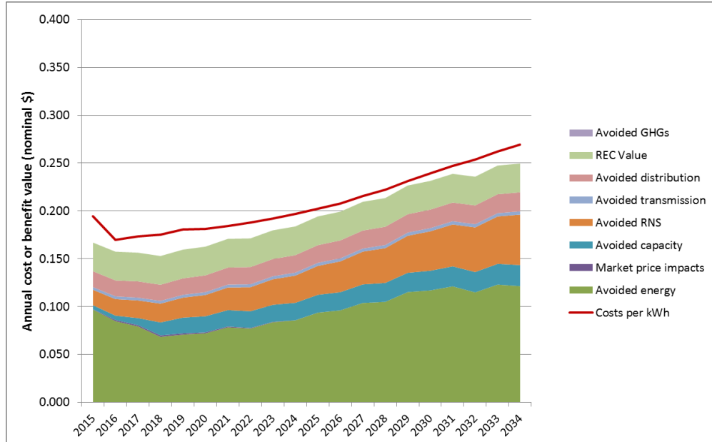
Exhibit 24. Per-kWh costs (red line) and benefits (colored areas) for a 100kW wind generator, group net metered, installed in 2015, from a ratepayer perspective.
